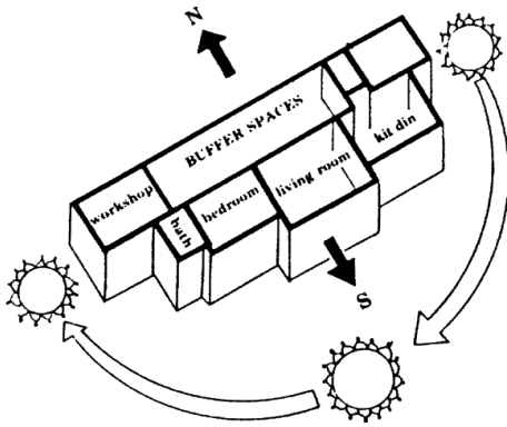
Figure 3. Buffer Spaces: Place rooms where they are compatible with the sun's path. Buffer spaces should be placed to the north.
